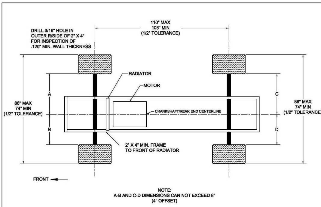
Chassis Diagram
